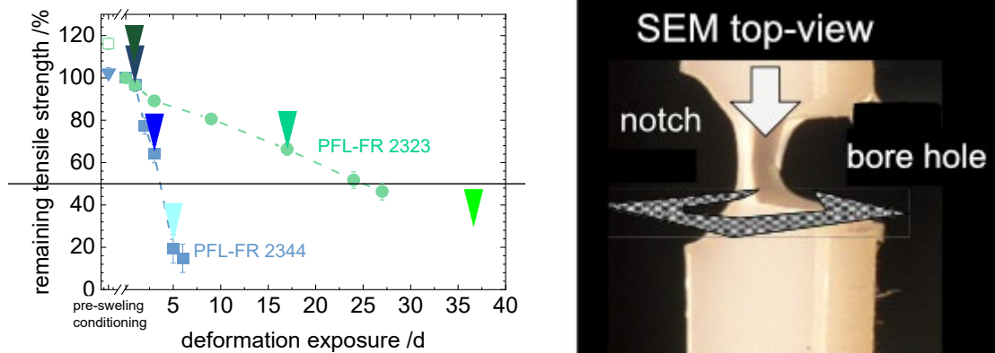
Fig. 5: Remaining tensile strength after immersion with pin in test liquid PFL-FR 2323 (green) und PFL-FR 2344 (blue) (left). Image of a specimen during tensile test (right) with sketched plane of subsequent fracture surface analysis by SEM.
