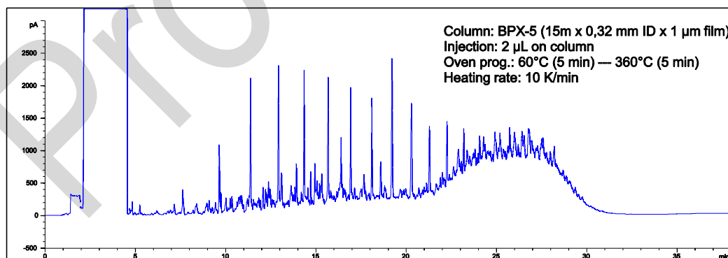
Fig.1: GC-FID chromatogram of diesel/lubricating oil calibration standard BAM-K010f
