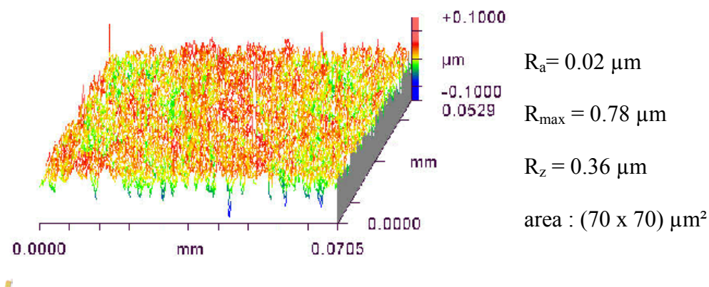
Fig. 8: WLI-topography (BAM-L104/056)
