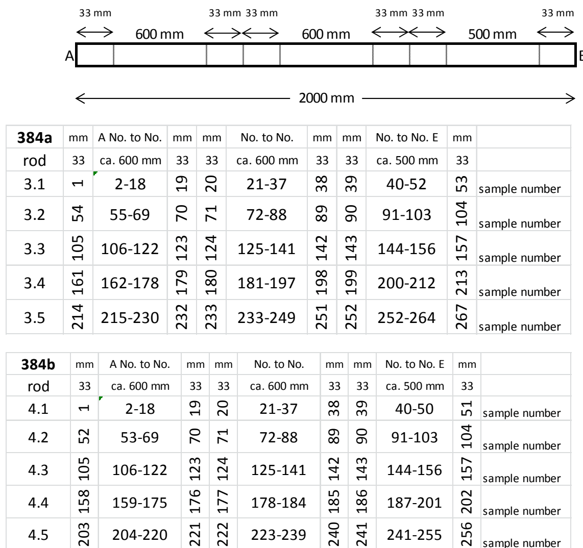
Figure 1: Cutting plans of pure copper reference materials
