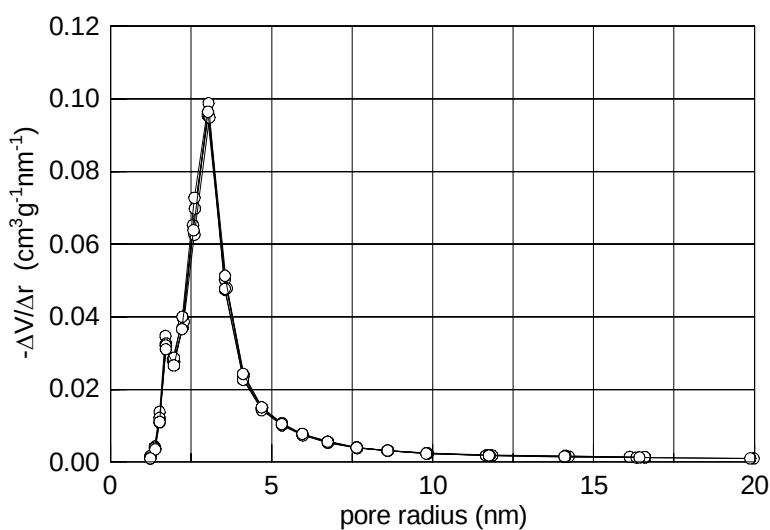
Figure 2: Pore size distribution of alumina type 150 (overlay of 9 measurements)
