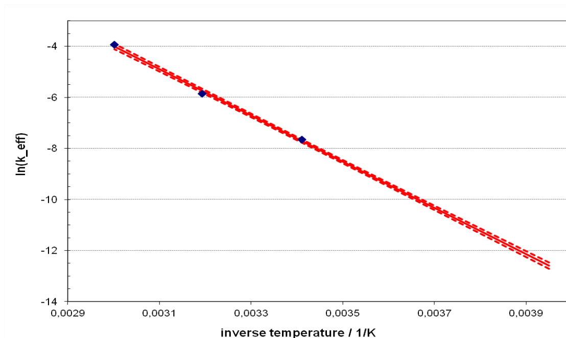
Figure 1: Dependence of the degradation rate of complex cyanides in CRM BAM-U114 on the inverse temperature (semi-logarithmic plot)
